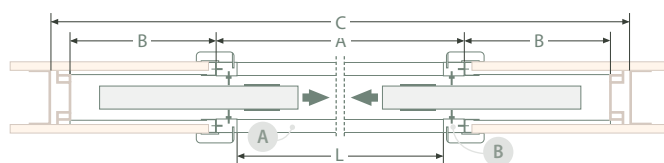
DIMENSIONS OF THE CASSETTE FOR DOUBLE SLIDING SYSTEM (mm)
