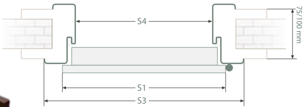
Covering assembly:
