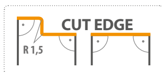
EDGE BANDING OF NON-REBATED DOOR LEAVES MADE IN THE CUT EDGE TECHNOLOGY (90°)
