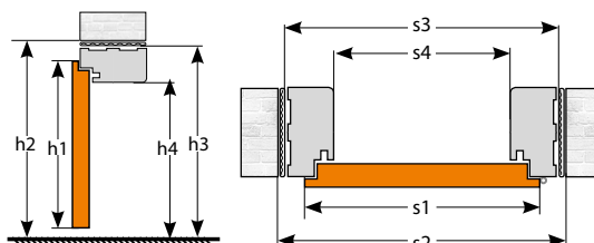
BLOCK DOOR FRAME + 2x FLAT ARCHITRAVE LO1 (10x60 mm) (OPTION AT EXTRA CHARGE)
